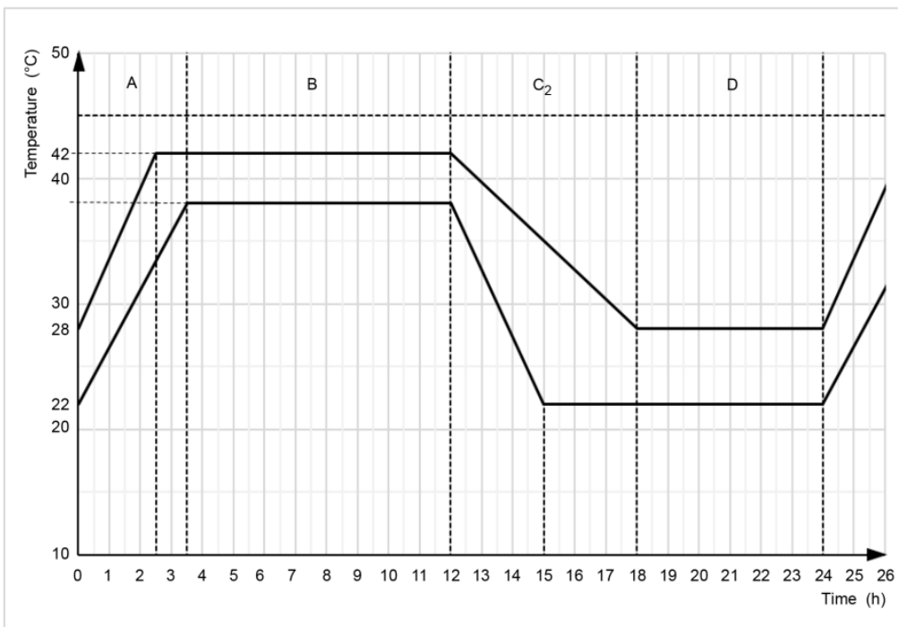
Figure 4 – Test Db – Test cycle – Variant 2, Method III
